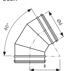
B60SX
