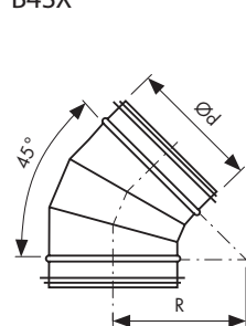
B45SX
